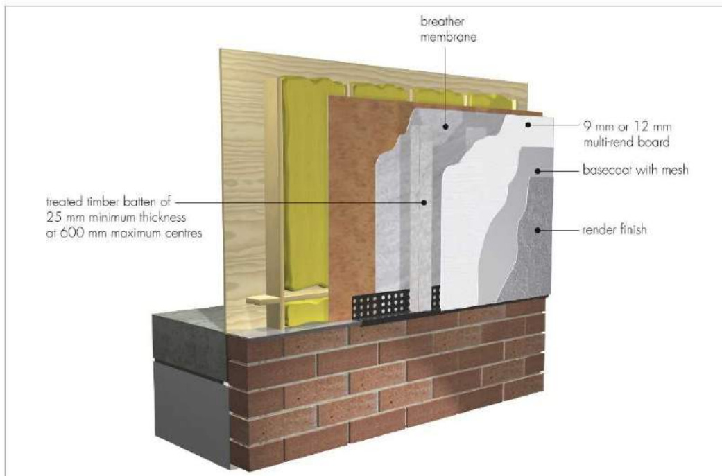
Figure 1 Multi-Rend system
